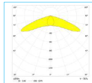
60x135°
