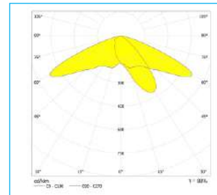
135x85°
